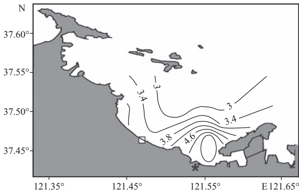
Fig.6 Spatial distributions of chl- a concentration (mg/m 3 ) “□” is the location of the estuary of Guangdang River; “*” is the location of the Xin'anhe Sewage Plant
